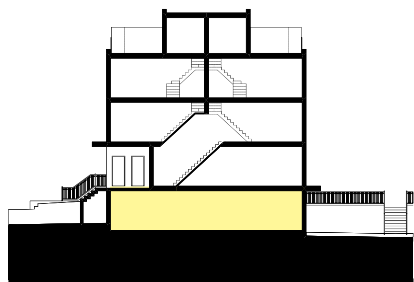
TYPICAL CROSS SECTION A
