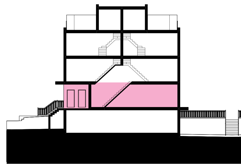
TYPICAL CROSS SECTION B
