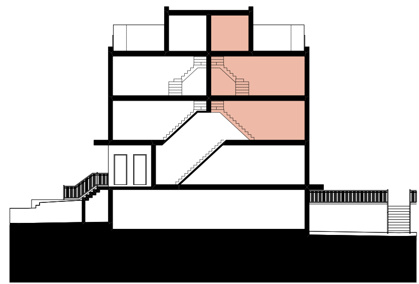
TYPICAL CROSS SECTION C
