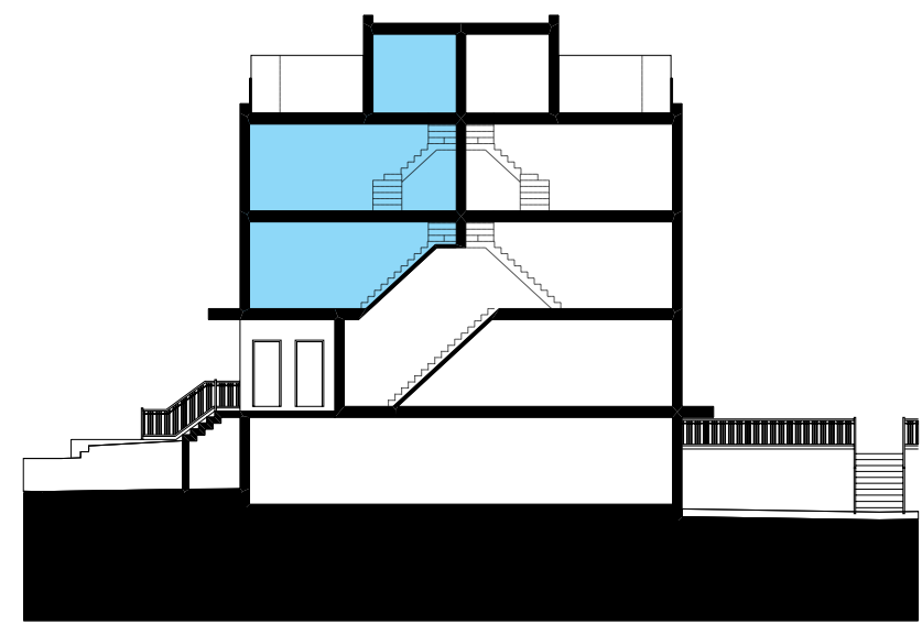
TYPICAL CROSS SECTION D
